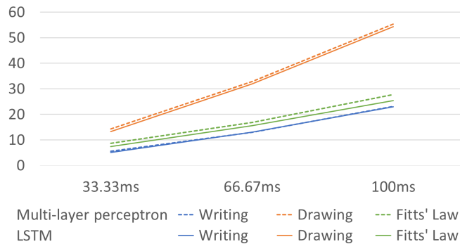
Figure 2: The development of the error for the three tasks with increasing extrapolation time.
