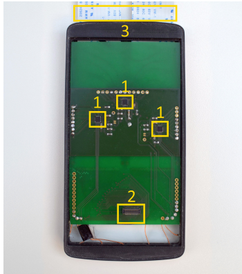
Figure 9: Case of the prototype holding a custom PCB comprising three MPR 121 (1), connectors for touchscreens (2), and flex cables (3) leading to the hardware box.
